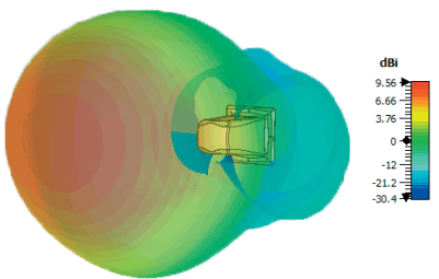
Typical 3D Pattern 3.6GHz**
