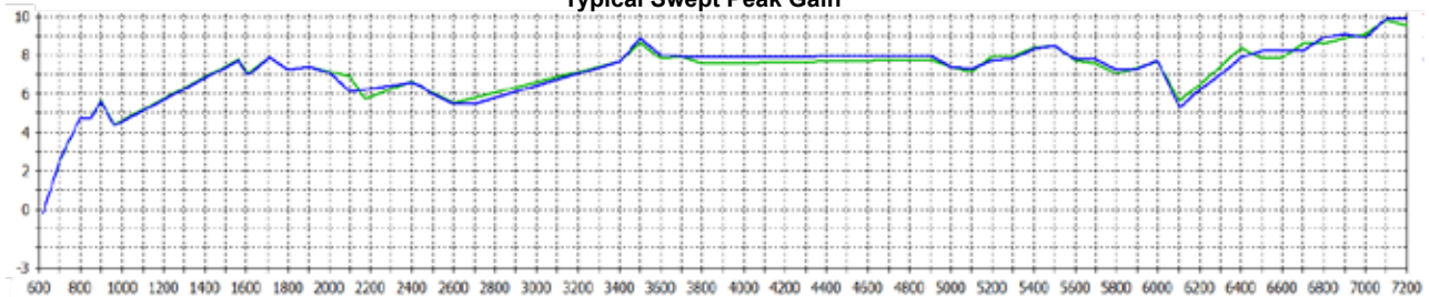
**Swept peak gain simulated in CST Microwave Studio for each element fed without cable loss on 600x600mm (2'x2') ground plane
