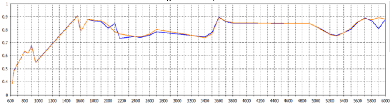
***Efficiency simulated in CST Microwave Studio for each element fed without cable loss on 600x600mm (2'x2') ground plane
