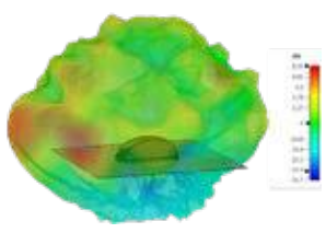
3D Plot Element 2 Side (5400 MHz)
