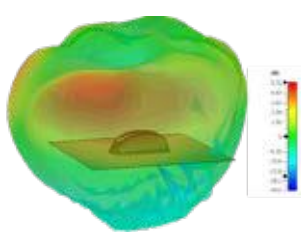
3D Plot Element 1 Side (5400 MHz)
