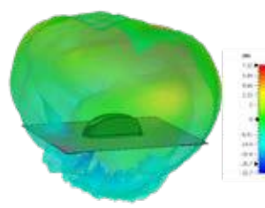
3D Plot Element 3 Side (5400 MHz)
