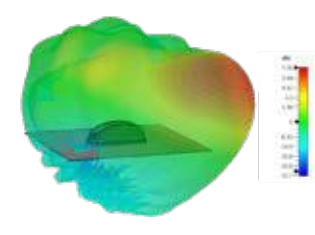
3D Plot Element 4 Side (5400 MHz)
