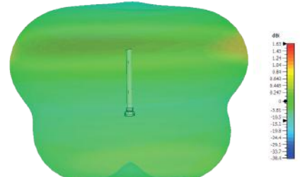
3D Plot Top Element (700MHz)
