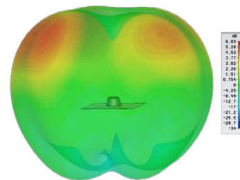
Typical 3D Pattern - Element 2 900MHz
