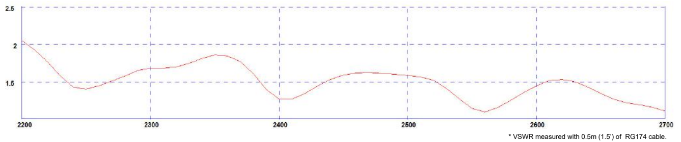
Typical VSWR WLAN element 3 - 2.4GHz*
