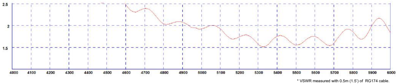
Typical VSWR WLAN element 3 - 5.8GHz*
