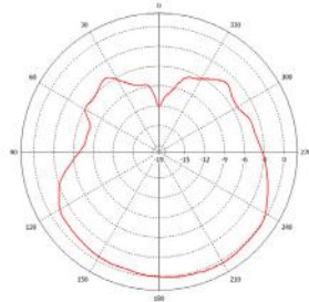
Typical H-Plane (2.7GHz)
