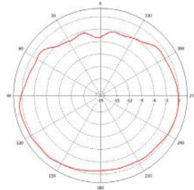
Typical H-Plane (1.9GHz)
