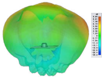
3D Pattern - WLAN (2.4GHz)
