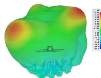
Typical 3D Pattern - Element 2 2600MHz
