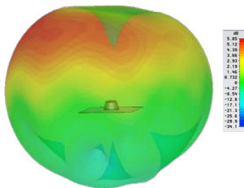
Typical 3D Pattern - Element 2 800MHz
