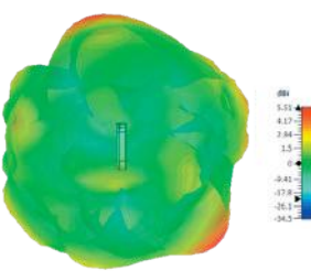
3D Plot Element C Side (5400 MHz)
